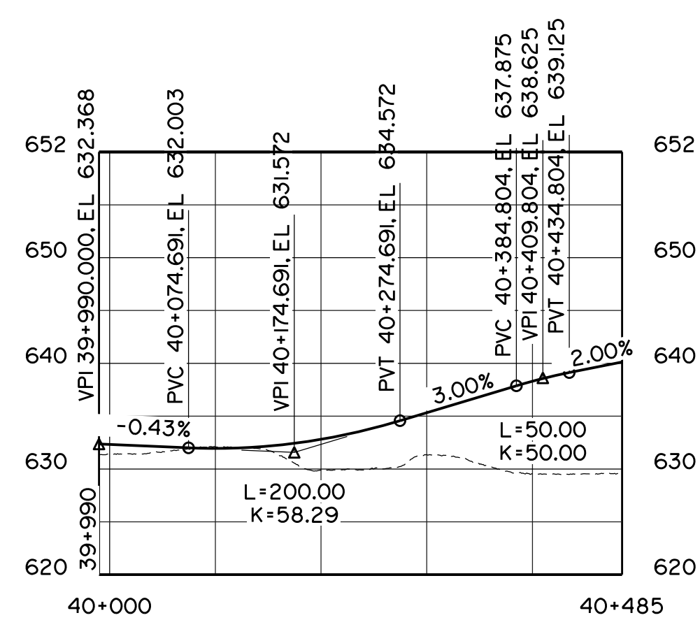
WB EXIT RAMP HOR 1: 5000 VERT 1: 500
