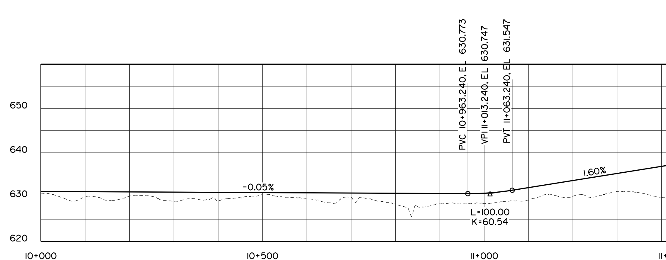
EB-NB LOOP RAMP
