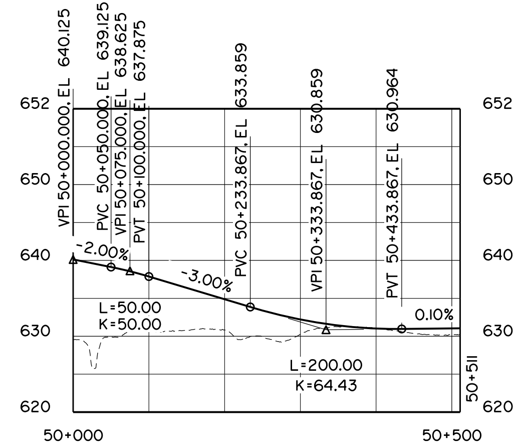
WB ENTRANCE RAMP HOR 1:5000 VERT 1:500
