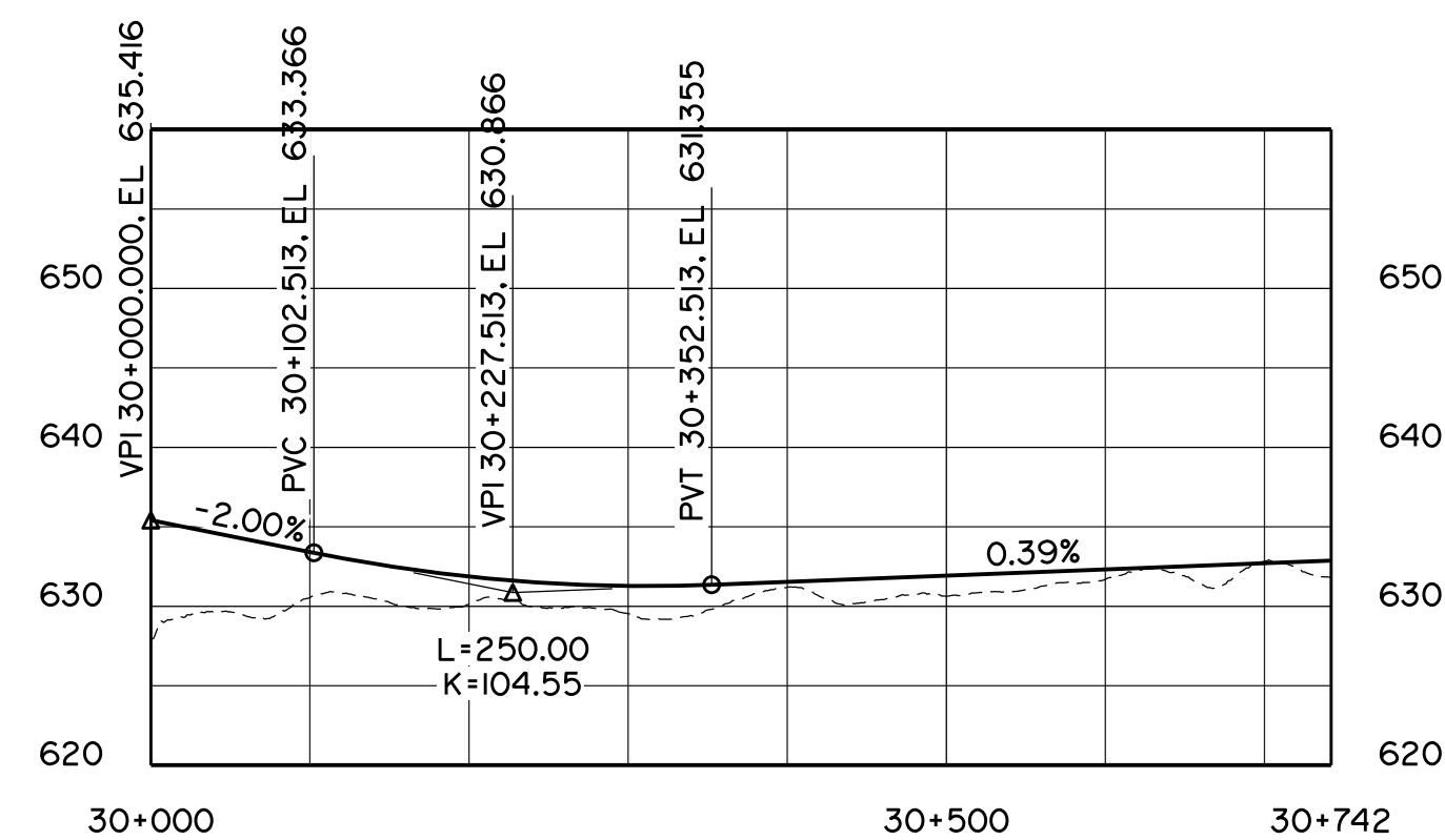
EB ENTRANCE RAMP HOR 1:5000 VERT 1:500
